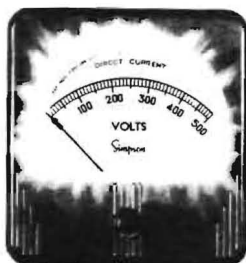
MODELS 27, 37, 57 ILLUMINATED 3 1/2" RECTANGULAR ACCURACY: 2% SCALE LENGTH: 1-5/16"
