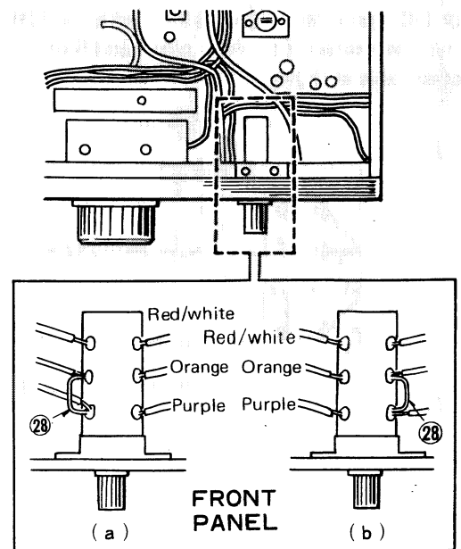
Fig 4 WWV Switch
