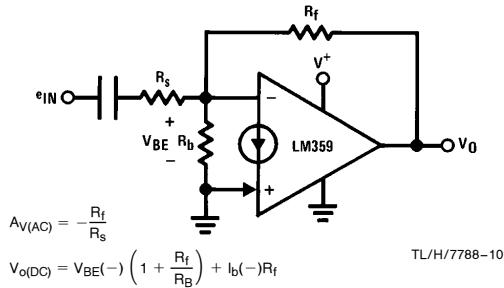
FIGURE 5. nV_{BE} Biasing
