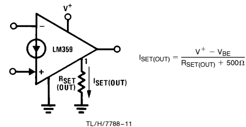
FIGURE 6. Establishing the Output Set Current
