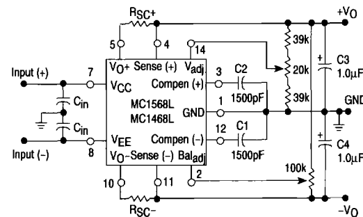
Figure 2. Voltage Adjust and Balance Adjust Circuit (14.5 V ≤ V O ≤ 20 V)
