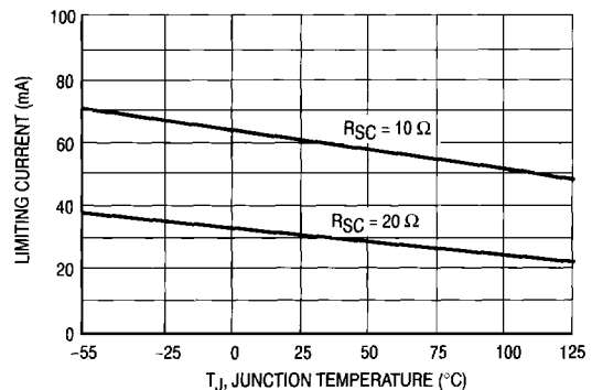
Figure 10. Current-Limiting Characteristics
