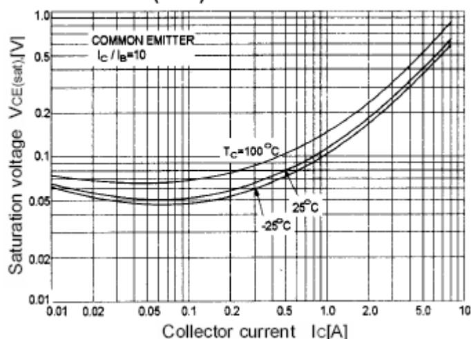
V_{CE(sat)} - I_C Characteristics
