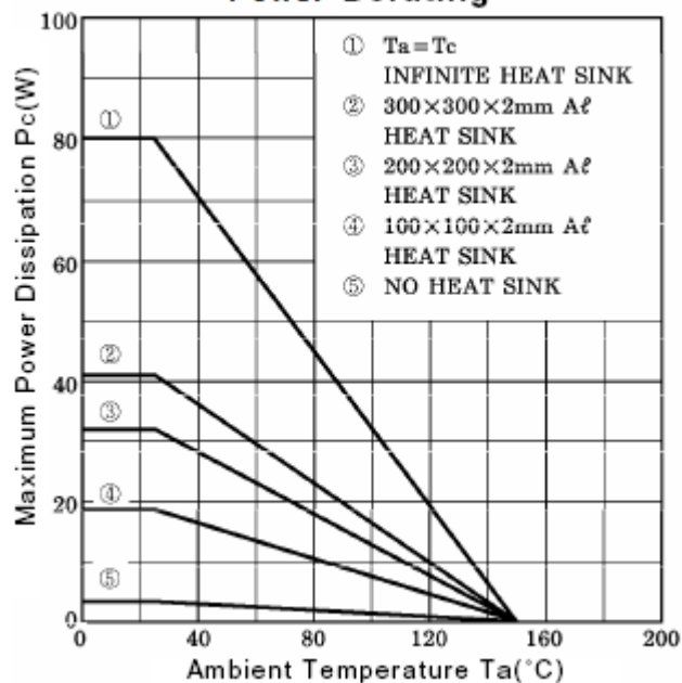
Power Derating
