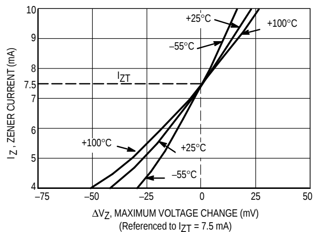
Figure 3. 1N821A Series
