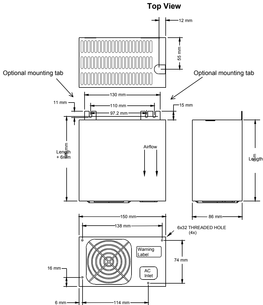
Figure 1: Enclosure Drawing
